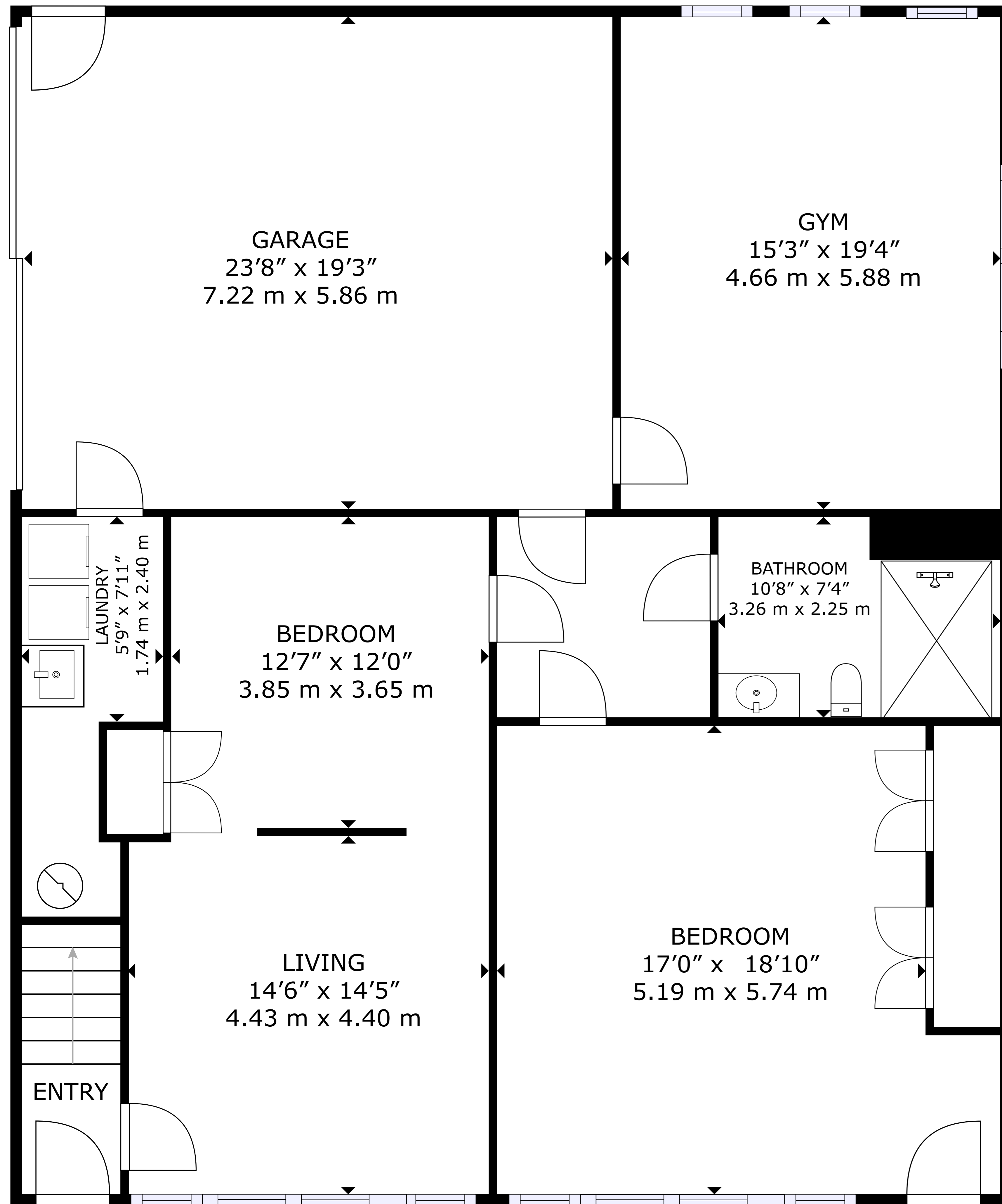
1ST FLOOR
